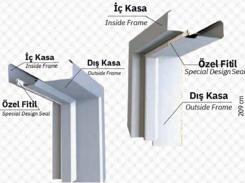
Kasa Kesit / Frame Details
